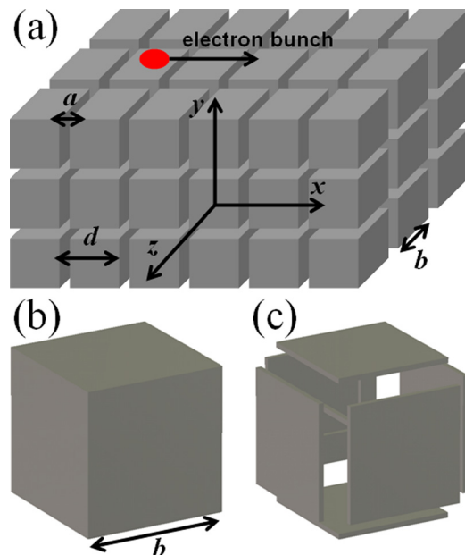
FIG. 1. (Color online) (a) Schematic model of the considered metamaterials with convection electrons. Unit cell structures for (b) type I and (c) type II metamaterials.
