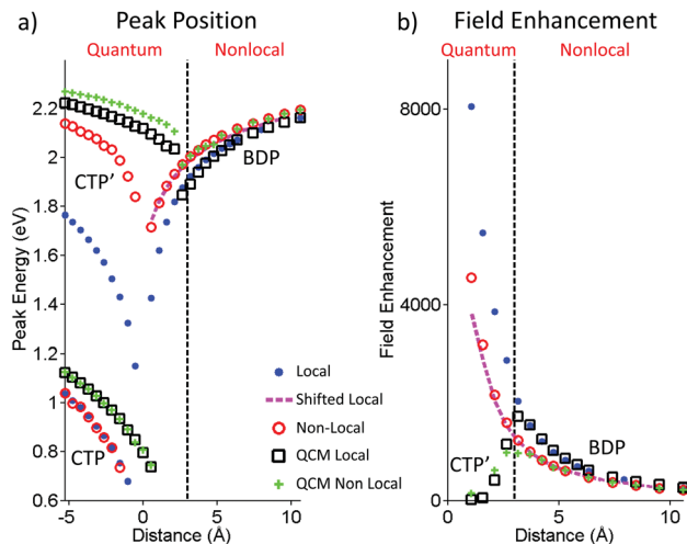
Fig. 8 Summary of the response predicted by the different models. (a) Energy of the extinction peaks of the main plasmon modes, and (b) maximum near field enhancement |E_g/E_0| at the center of the gap as a function of separation distance, for local classical (blue dot), nonlocal classical (red open circle for hydrodynamical model and magenta dashed line for distance rescaling), local QCM (black open square) and nonlocal QCM (green +, calculated with the hydrodynamical formalism). The values correspond to those indicated by circles in Fig. 6 and 7. The vertical dashed line corresponds to d = 3.0 Å and approximately separates the distance ranges where either the quantum-induced charge transfer or nonlocal effects dominate the response, as indicated at the top of the figure. The labels of the plasmon peaks refer to the Bonding Dimer Plasmon (BDP) and to the two lowest-energy Charge Transfer Plasmons (CTP and CTP').
