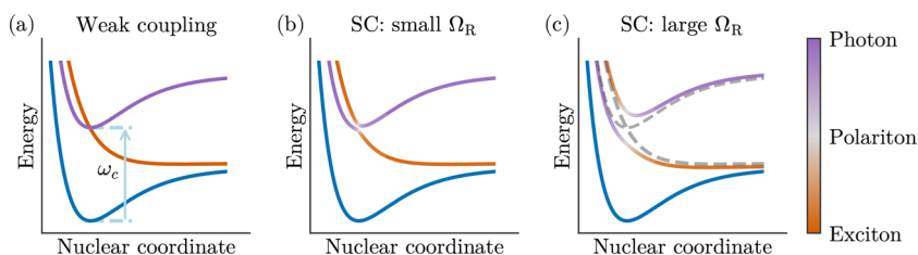
Figure 1. Conceptual potential energy surfaces for a single molecule and a light mode in (a) weak coupling and (b, c) strong coupling for different coupling strengths. The color represents the photonic fraction of the state from purely excitonic (orange) through polaritonic (light gray) to purely photonic (purple).
