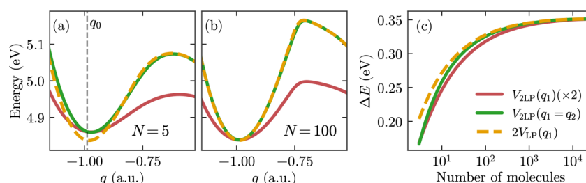
Figure 7. (a, b) Comparison of the PoPEs in the double-excitation subspace for motion of one molecule (red line) and two molecules (green line) and twice the lower PoPEs in the single-excitation subspace for motion of one molecule (orange dashed line), for N = 5 and N = 100 coupled molecules, respectively. (c) Dependence of the energy barrier for double photoisomerization with the number of molecules for the reaction paths corresponding to the PoPEs in (a) and (b).
