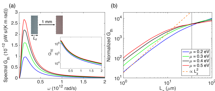
Figure 2. (a) Spectral thermal conductance as a function of the radiation frequency for a system composed of two graphene flakes of length L_z = 10 \mu\text{m} , \mathcal{E}_s = 10^{-4} eV, and a gap d = 1 mm (see upper inset). The different lines correspond to distinct chemical potentials (see legend in (b)), and the temperature is 300 K. The lower inset shows the corresponding absorption efficiency Q_{\text{TE}}(\omega) in the same frequency range as the spectral conductance. (b) Total thermal conductance G_{\text{th}} , normalized by the blackbody results, for the same system as in panel (a) and plotted as a function of L_z for different chemical potentials. The dashed orange line is proportional to L_z^2 . The vertical dotted line indicates approximately the length at which the conductance for \mu = 0.5 eV starts to saturate (see text). Let us stress that these normalized results do not depend on the gap d as long as d is much larger than the thermal wavelength.
