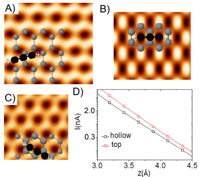
Figure 6. Calculated STM images obtained with our graphitic tip (placed at 4.5 Å) for three different relative orientations related to the graphene layer and indicated in the corresponding superimposed ball and stick models (black spheres represents the tip atoms). (A) Shows a honeycomb pattern, (B) a triangular-like pattern and (C) a hexagonal pattern with two asymmetric maxima. (D) I(Z) curves calculated including the MS effects over a maximum (red circles) and a depression (black squares) of the STM image shown in (A). The image remains unchanged with this tip.
