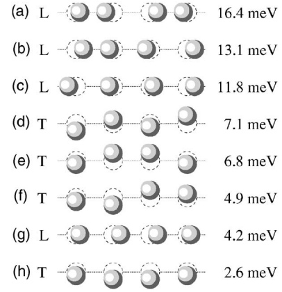
FIG. 7. A sketch of the vibrational eigenmodes of a linear four-atom gold wire, with energies corresponding to d=2.62 \text{ \AA} in geometry A. The longitudinal modes (L) are all nondegenerate, whereas the transverse modes (T) are all doubly degenerate.
