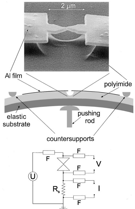
Fig. 2. Three point bending mechanism. The distance between the two counter-supports is 12 \text{ mm} , and the substrate is 0.3 \text{ mm} thick. The micrograph shows a suspended Al microbridge. The insulating polyimide layer was etched to free the bridge from the substrate. The third panel displays the wiring of the experimental setup.
