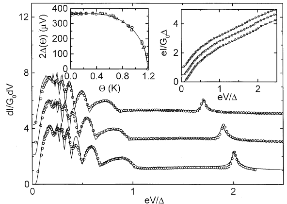
Fig. 3. Differential conductance dI/dV as a function of voltage measured at \Theta = 47 mK (bottom), 640 mK (middle), and 810 mK (top) for a contact with total conductance D = 1.008 . The two upper curves are offset by 2 each. The solid lines are fits using the same transmission ensemble \{T_1 = 0.900, T_2 = 0.108\} for all three temperatures. Right inset: corresponding I - V s offset by 0.5 each. Left inset: position of the m = 1 maximum in the dI/dV curves. Data has been taken on three different contacts with G varying from 1 to 2 G_0 . The line is the temperature dependence of the superconducting gap according to BCS theory for \Delta(\Theta = 0) = 184 \mu\text{V} .
