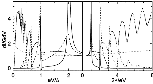
Fig. 4. Calculated dI/dV characteristics (normalized to the conductance) of a single channel quantum point contact for transmission 0.1 (solid), 0.6 (dashed), 0.9 (dash-dotted), 1.0 (dotted) as a function of eV/\Delta (left panel) and m' = 2\Delta/eV (right panel). The maximum of the curve for T = 0.1 arrives at 12.6G . The amplitude, the shape and the exact position of the individual maxima depend on the transmission. Only for small T the maxima are close to V = 2\Delta/me , for higher transmission they are shifted to lower voltages. The subgap structure is most pronounced for intermediate T .
