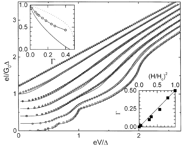
Fig. 5. Measured (symbols) and calculated (lines) I - V s of trace (d) of Fig. 1 with transmission set \{0.519, 0.253, 0.106\} for magnetic fields of \mu_0 H = 0, 2.1, 5.4, 5.9, 7.7, 9.1 and 10.9 mT (from bottom to top). The curves with magnetic field are offset by 0.2 each. Left inset: pair amplitude \Delta (dotted), spectral gap \Omega (solid) (according to [34]) and position of the m = 1 maximum of the corresponding calculated dI/dV s (symbols) in units of the gap parameter at zero field as a function of the pair breaking parameter \Gamma . Right inset: Pair breaking parameter \Gamma used for calculating the I - V s and dI/dV s as a function of applied field (symbols) and prediction according to [32,24] (line). The I - V at H = 0 was measured at the beginning and the end of the series of measurements and the \{T_n\} was found to be reproducible. The critical field at the measuring temperature of \Theta = 25 mK was determined to be \mu_0 H_c = 10.2 mT.
