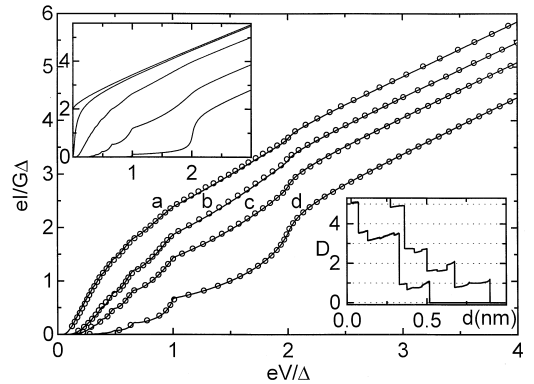
Fig. 1. Measured I - V curves (symbols) of four different atomic contacts with G \simeq 0.9G_0 at \Theta \leq 50 mK and best numerical fits (lines). The \{T_n\} and total transmissions D obtained from the fits are: (a) \{0.900, 0.108\} , D = 1.008 ; (b) \{0.802, 0.074\} , D = 0.876 ; (c) \{0.747, 0.168, 0.036\} , D = 0.951 ; (d) \{0.519, 0.253, 0.106\} , D = 0.878 . Current and voltage are in reduced units, the current axis is normalized with respect to the total conductance measured by the slope of the I - V at high voltages eV > 5\Delta . Not all measured data points are shown. The measured gap was \Delta/e = (184 \pm 2) \mu V. Left inset: Theoretical I - V s for a single-channel superconducting contact for different values of T (from bottom to top: 0.1, 0.6, 0.9, 1) after [11]. Right inset: typical total transmission traces measured as a function of the electrode distance d at eV > 5\Delta , while opening the contact at around 6 pm/s. The d -axis has been calibrated by the exponential behavior in the tunnel regime.
