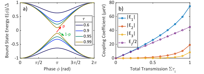
Fig. 4 Energy-phase relation and coupling coefficients. a Andreev-bound state relation for high transmissions. As the gap closes, the probability for transitions between branches (non-adiabatic processes) becomes more likely. b Absolute value of the coupling coefficients |E_m| at different transmissions in comparison to the coupling coefficient of the linear Ambegaokar-Baratoff model ( E_j/2 ).
