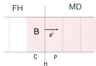
FIG. 1. (Color online) Geometry of the domain decomposition used in the hybrid scheme. Fluctuating hydrodynamics and molecular dynamics domains, labeled as FH and MD, respectively, are separated by the hybrid interface H . The shaded area corresponds to the particle region MD+B, where B is the particle buffer . However, the total system is uniquely determined by MD+FH.
