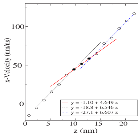
FIG. 10. (Color online) Calculation of the shear viscosity of argon at \rho = 0.6 \text{ gr/mol/\AA}^3 and T = 300 \text{ K} using the hybrid code. The guess value for the viscosity at the FH domain is \eta_{\text{FH}} = 5.31 \times 10^{-5} \text{ Pa s} ; the slopes (shear rates) at the MD and FH domain (indicated in the figure) provide \eta_{\text{MD}} = (\dot{\gamma}_{\text{FH}} / \dot{\gamma}_{\text{MD}}) \eta_{\text{FH}} = 7.50 \times 10^{-5} \text{ Pa s} .
