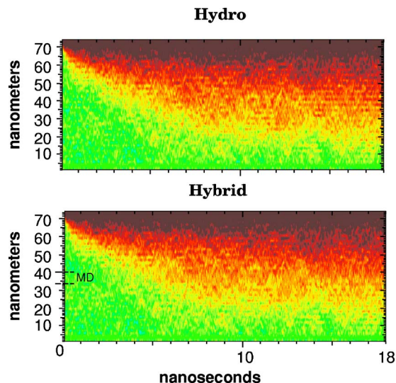
FIG. 6. (Color online) Spatiotemporal diagram showing the startup of a Couette flow. “Hydro” denotes results from the fluctuating hydrodynamic model (FH) and “Hybrid” from the hybrid MD-FH simulation (the MD region is indicated between the horizontal dashed lines). The velocity imposed at the upper wall is 1 \text{ \AA}/\text{ps} and the bottom wall is at rest.
