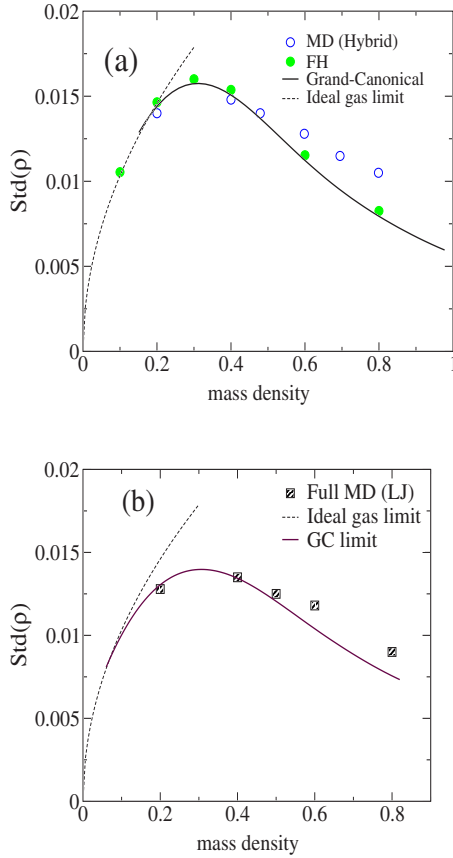
FIG. 4. (Color online) (a) Standard deviation of the mass density versus the mean mass density for argon. The result for the grand-canonical ensemble is [\rho k_B T / (V_c c_T^2)]^{1/2} , where c_T^2 = (\partial P / \partial \rho)_T is the squared isothermal sound velocity. Results at FH and MD cells are shown. (b) Results obtained in full MD simulations using large simulation boxes (see text). The argon model used in (b) (simple LJ [36]) has a lower compressibility with respect to (a) arising from a pressure excess of \delta p(\rho) = 250\rho^2 bar; see Fig. 3. Density is given in units of \text{gr/mol}/\text{\AA}^3 .
