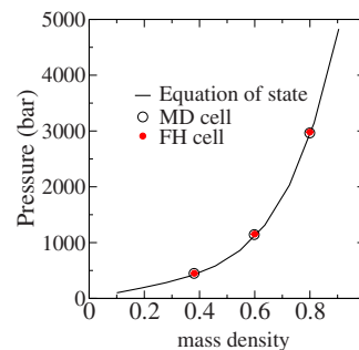
FIG. 3. (Color online) The mean pressure versus the mean mass density \rho for argon. The equation of state is that of Johnson et al. [36] corrected for the contribution of the switched potential added in MD code ( P_{\text{switch}}=-250.8\rho^2 bar). Density is given in \text{gr mol}^{-1} \text{\AA}^{-3} ( =1.687 \text{gr/cm}^3 ).
