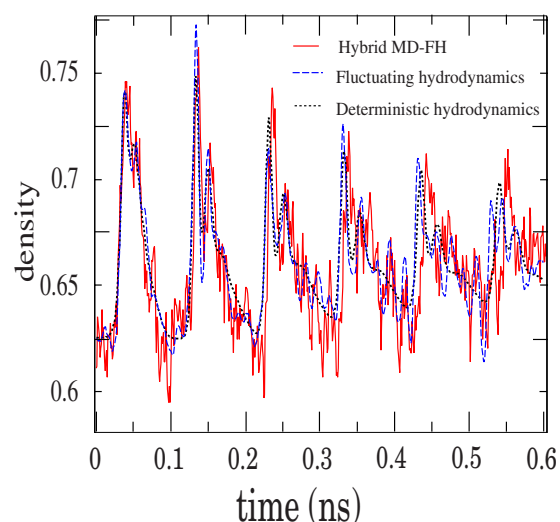
FIG. 9. (Color online) The temporal evolution of the density at the center MD cell in a simulation of a sound wave reflecting within a closed box (argon at T=300 \text{ K} ). Comparison is made between the hybrid solution and those obtained using deterministic and fluctuating hydrodynamics with similar initial conditions. Density in units of \text{gr}/(\text{mol } \text{\AA}^3) .
