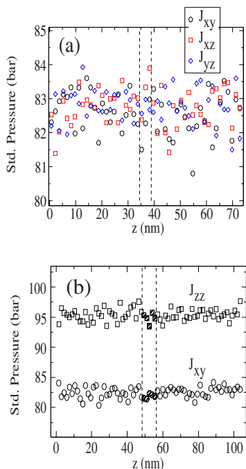
FIG. 5. (Color online) The standard deviation of the pressure tensor components at different cell locations. Results correspond to argon at \rho=0.6 gr/mol/ \text{\AA}^3 and T=300 K. Cells pertaining to the MD domain are located between dashed lines. Coupling time is \Delta t_c=250 fs and n_{\text{FH}}=5 and n_{\text{MD}}=25 . (a) Results for the off-diagonal components of the pressure tensor using the mesoscopic approach for the pressure tensor within the MD domain (see text). (b) Results for diagonal and off diagonal components of the stress tensor obtained when the microscopic stress tensor [Eq. (15)] is used at the MD domain.
