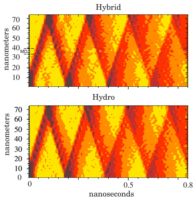
FIG. 8. (Color online) Spatiotemporal diagram showing the evolution of a density wave within a closed box. Comparison is made between results from the fluctuating hydrodynamic model (“Hydro,” at bottom) and from the hybrid MD-FH model (“Hybrid,” at top). The MD region is located at the center of the box, as indicated. The system is divided in 49 control cells, aligned in z direction, with dimensions 50 \times 50 \times 15 \text{ \AA}^3 . The mean density is about \rho = 0.6 \text{ gr}/(\text{mol } \text{\AA}^3) . Upon the initial perturbation the maximum and minimum densities are 0.85 and 0.55 \text{ gr}/(\text{mol } \text{\AA}^3) , providing an initial Mach number ( \text{Ma}^2 \sim \Delta\rho/\rho ) of about \text{Ma}=0.7 .
