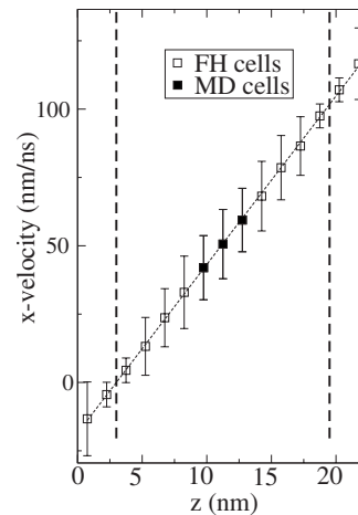
FIG. 7. Steady solution of the Couette flow velocity. Error bars indicate the standard deviation of the velocity within each cell, which corresponds to that of argon at \rho=0.6 gr/mol/ \text{\AA}^3 and temperature T=300 K. The viscosity, \eta=7.50 \times 10^{-5} Pa s was previously calibrated using the hybrid setup (see Appendix D 2).
