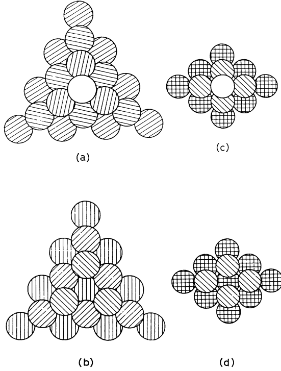
FIG. 1. Simulated STM tips studied in this work; (a) sharp (111); (b) flat (111); (c) sharp (110); and (d) flat (110).
