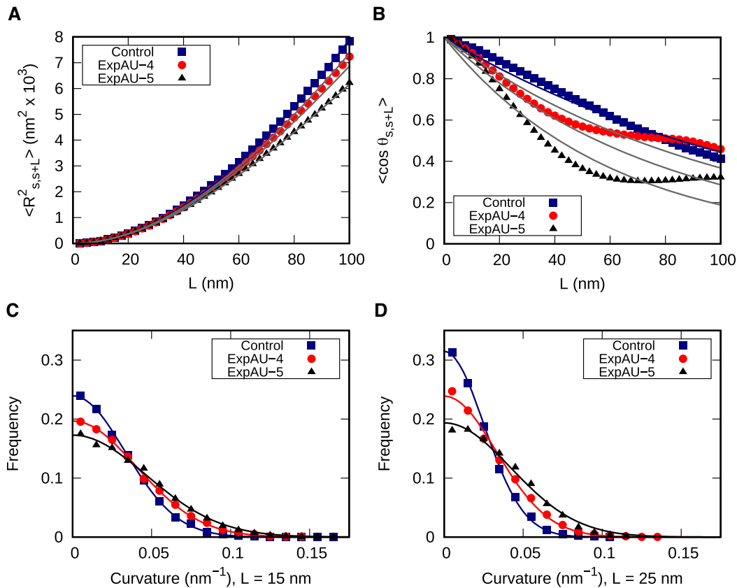
Figure 5. Experimental quantification of dsRNA bending induced by AU-tracts. Mean squared end-to-end distance (A) and mean cosine of the tangents (B) plotted as a function of the contour distance between two points. The blue solid line is a fit of the control data to the WLC equations (Equation (1) for panel A, and Equation (2) for panel B), which yielded P = 66 \pm 1 nm and P = 62 \pm 1 nm for the \langle R_{s,s+L}^2 \rangle and \langle \cos \theta_{s,s+L} \rangle data, respectively. To guide the eye, theoretical WLC curves are included with persistence lengths of 30, 40 and 50 nm (bottom-up in both panels). Histograms of curvature distributions for fixed contour lengths of 15 nm (C) and 25 nm (D), showing the relative frequency of different curvature values. The distributions were fitted to Gaussian functions (solid lines). The standard deviation parameters obtained from these Gaussian fits are presented in Table 2.
